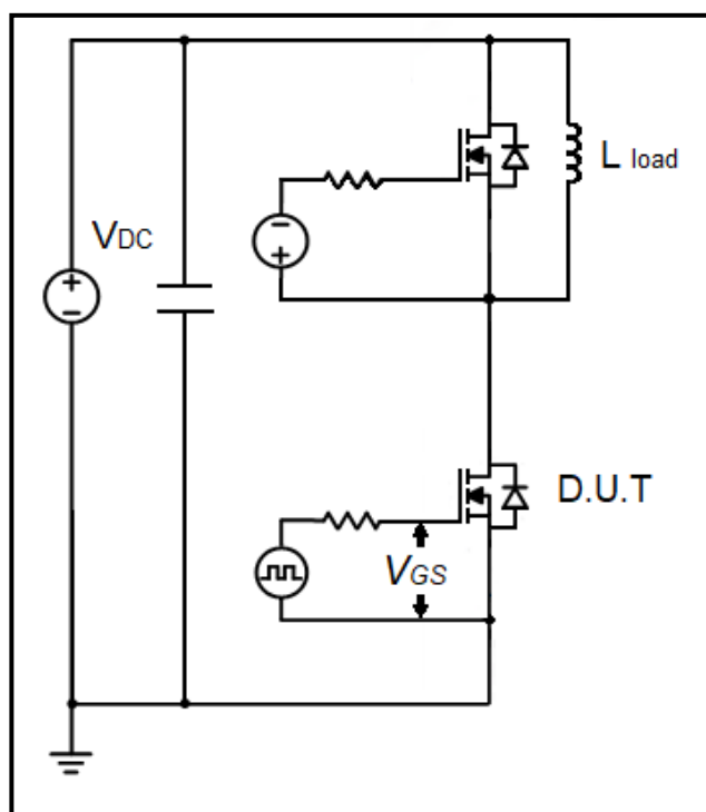
Figure 30. Clamped inductive switching waveform test circuit
