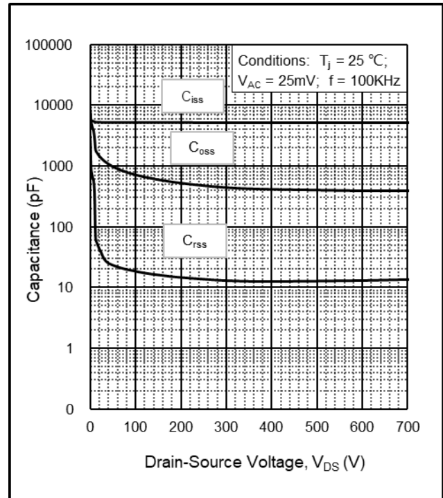
Figure 18. Capacitance vs. drain-source voltage (0 - 700V)
