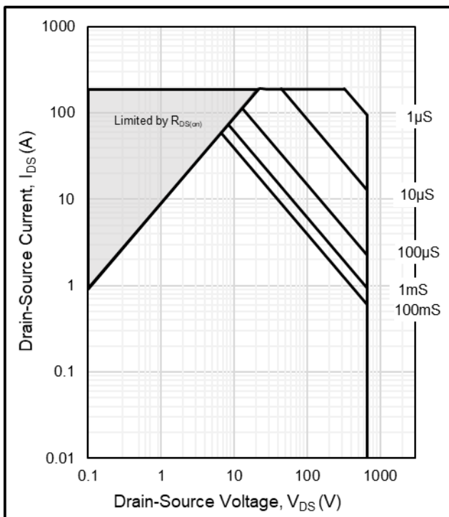
Figure 23. Safe Operating Area
