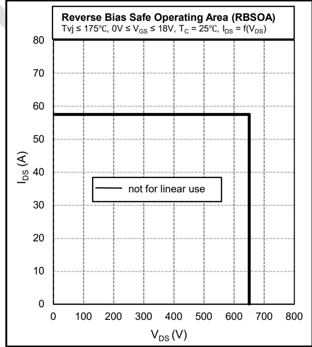
Figure 24. Reverse Bias Safe Operating Area
