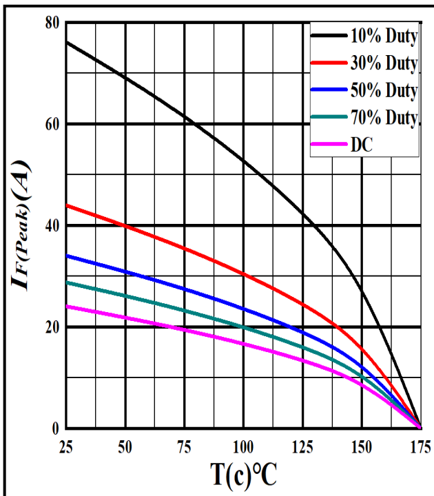
Figure 3. Current derating
