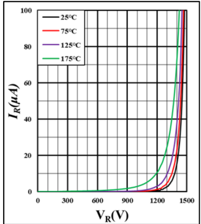
Figure 2. Reverse characteristics
