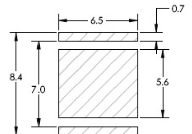
Figure 1: Recommended solder pad layout and size for SST-50. All dimensions in mm.
