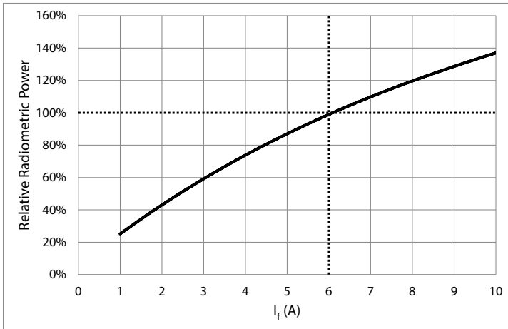
Relative Power vs Forward Current, T_{HS} = 40^{\circ}\text{C}
