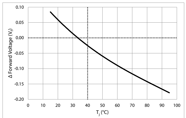
Rel. Forward Voltage vs Junction Temperature
