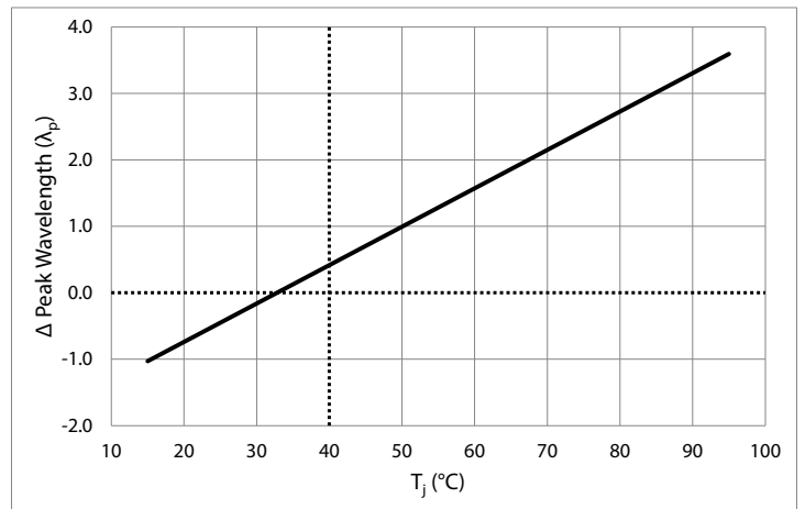
Rel. Peak Wavelength vs Junction Temperature
