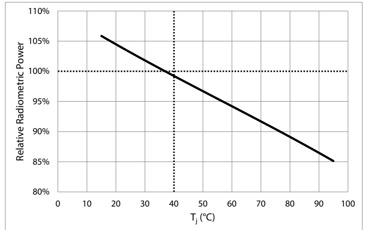
Relative Power vs Junction Temperature
