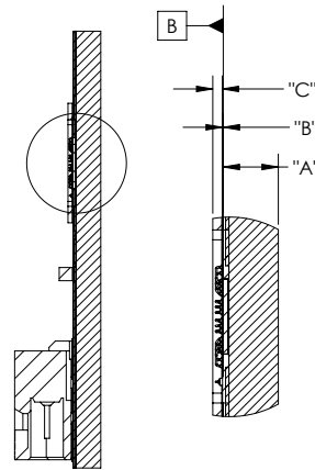
SECTION E-E
