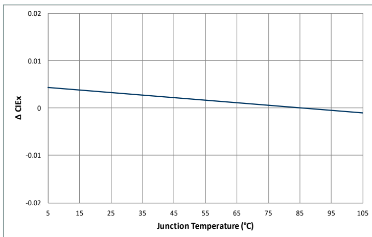
Change in CIE_x vs. Junction Temp. (3000K, 90CRI)
