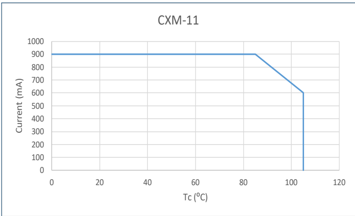
Derating Curves
