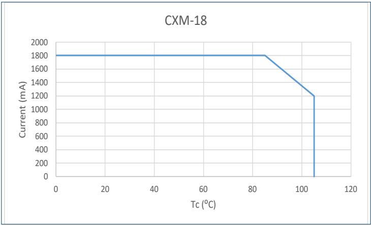
Derating Curves
