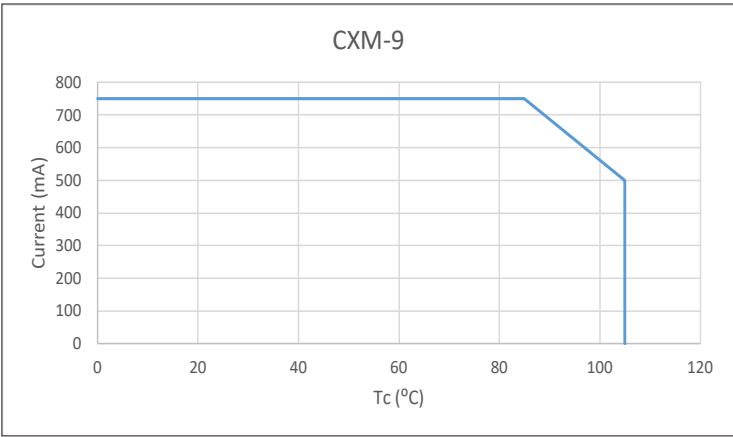
Derating Curves
