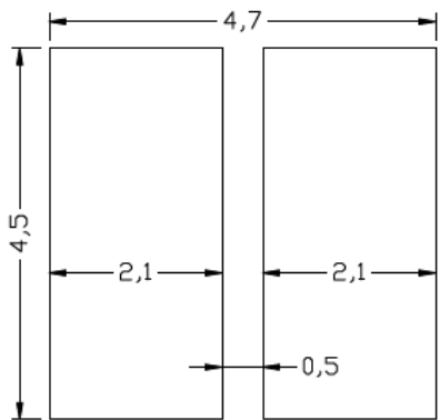
Recommended Solder Pad Design
