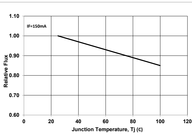
Tj-----Relative Luminous Flux
