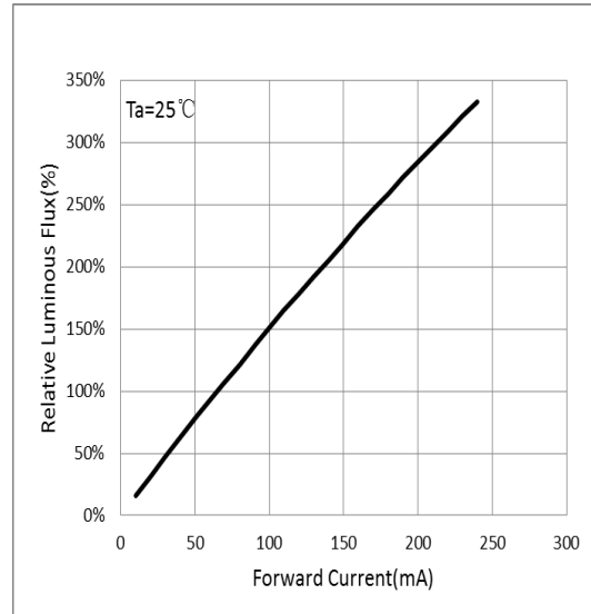
I_f ----- Relative Luminous flux
