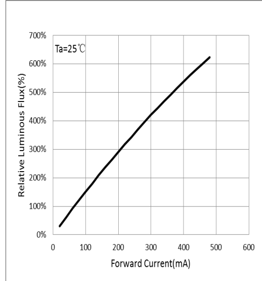
I_f ---- Relative Luminous flux
