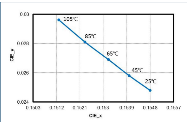
Color B Relative Chromaticity vs Temperature
