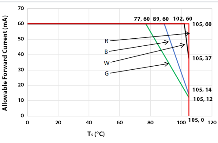
Allowable Forward Current vs Temperature
