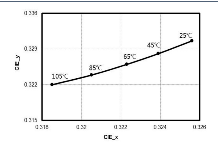
Color G Relative Chromaticity vs Temperature
