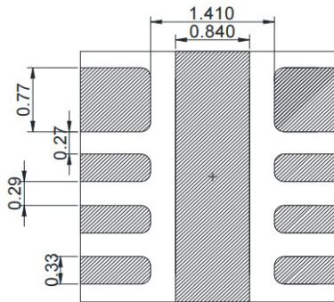
Soldering patterns
