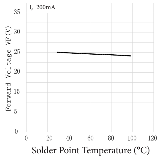
T_s ---- Forward Voltage
