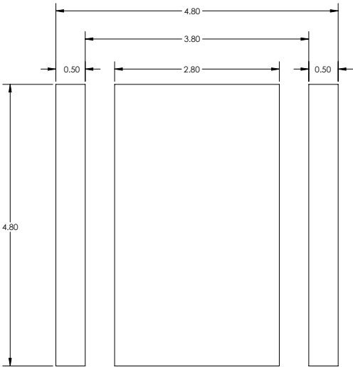
RECOMMENDED PCB SOLDER PAD DESIGN
