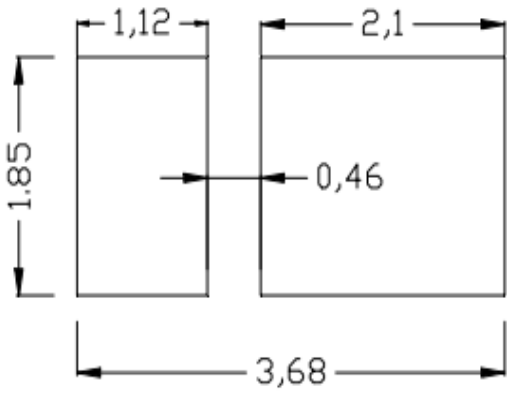
Recommended Solder Pad Design
