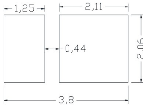
Recommended Solder Pad Design
