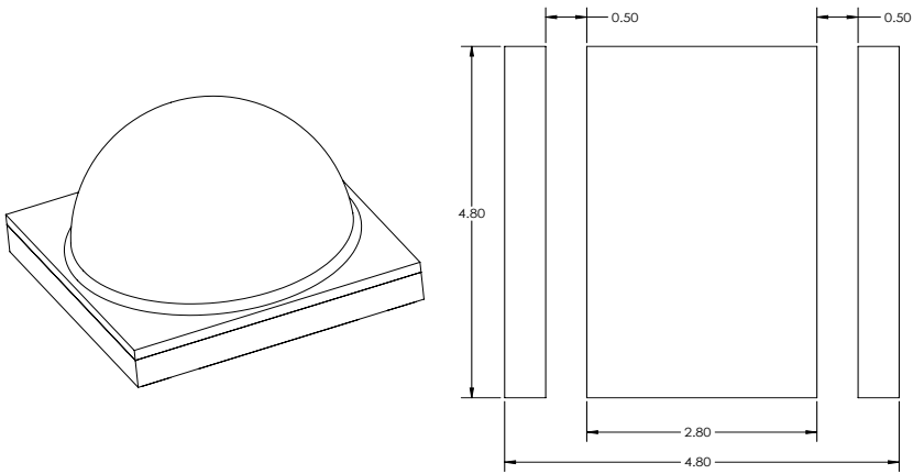
RECOMMENDED PCB SOLDER PAD
