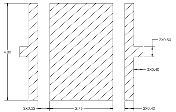
RECOMMENDED STENCIL PATTERN
